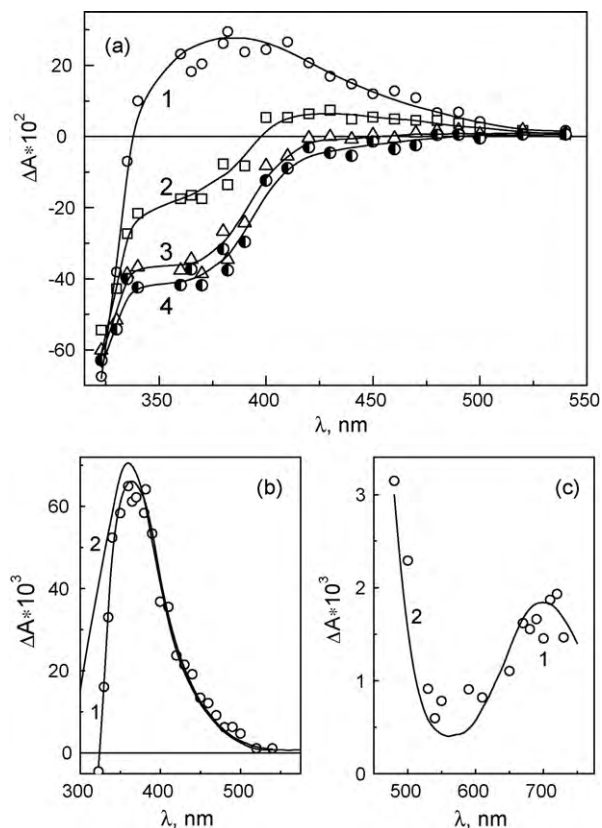
Fig. 4. Intermediate absorption spectra caused by laser flash photolysis (308 nm) of aqueous \text{PtBr}_6^{2-} solution ( 4.2 \times 10^{-5} M) in the presence of 4 M NaBr (a) curves 1–4 correspond to 0, 10, 50, 175 \mu\text{s} after laser pulse. (b) 1 – difference in spectra 1 and 4 shown in (a), 2 – spectrum of \text{Br}_2^{\bullet-} radical anion [15]. (c) 1 – intermediate absorption after the laser pulse in the red spectral region, 2 – \text{Br}_2^{\bullet-} spectrum.
