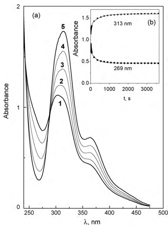
Fig. 3. Thermal reaction after the photolysis of aqueous \text{PtBr}_6^{2-} solution ( 9.3 \times 10^{-5} M) in the presence of 4 M NaBr. (a) curve 5 – spectrum of the initial complex; curves 1–4 correspond to 0; 30; 180; 3780 s after irradiation. (b) Kinetic curves (dots) and two-exponential fits (full lines).
