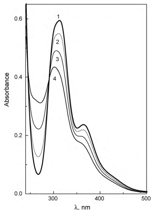
Fig. 2. Stationary photolysis of \text{PtBr}_6^{2-} complex ( 3.5 \times 10^{-5} M) in aqueous solutions with addition of 1 M NaBr. Excitation by XeCl laser pulses (308 nm). Curves 1–4 correspond to 0, 3, 9, 20 laser pulses.
