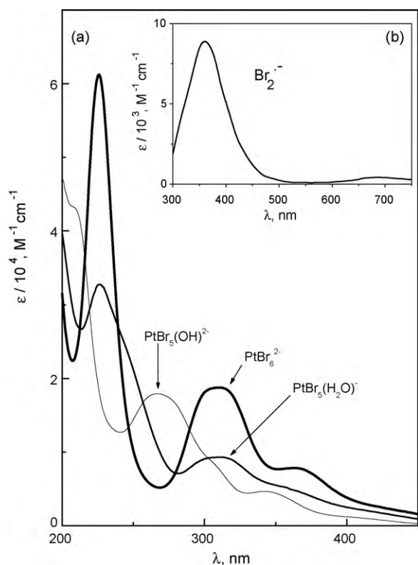
Fig. 1. UV absorption spectra of Pt(IV) complexes (a) and \text{Br}_2^{\bullet-} radical anion (b) [15] in aqueous solutions. Spectra of \text{PtBr}_5(\text{H}_2\text{O})^- and \text{PtBr}_5(\text{OH})^{2-} complexes are taken from [7].
